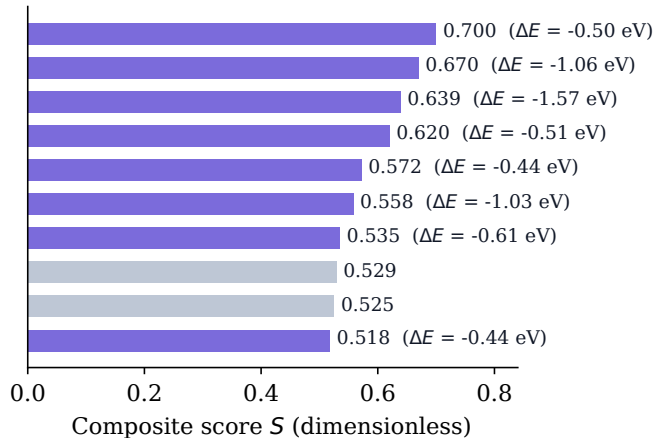
(b) Composite ranking
