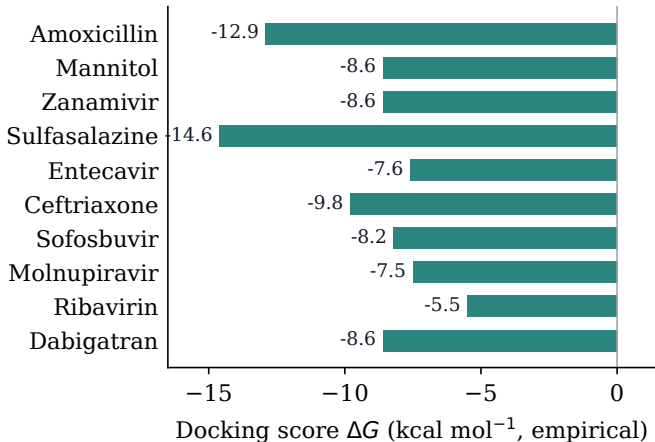
(a) Docking scores
