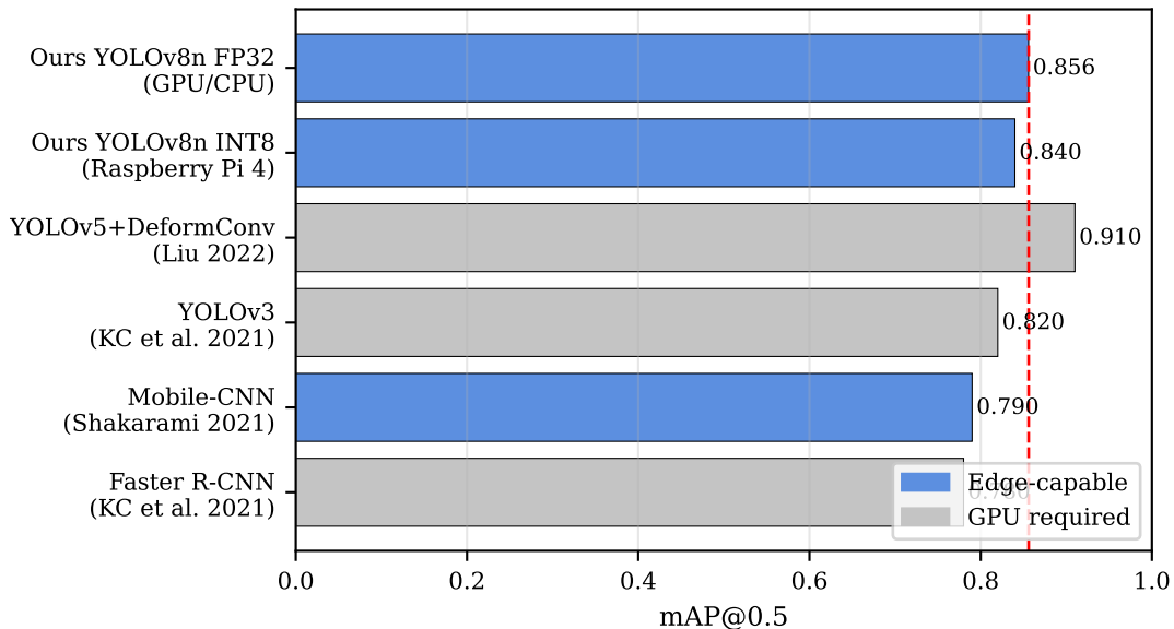
mAP@0.5 on BCCD / PBS Benchmarks
