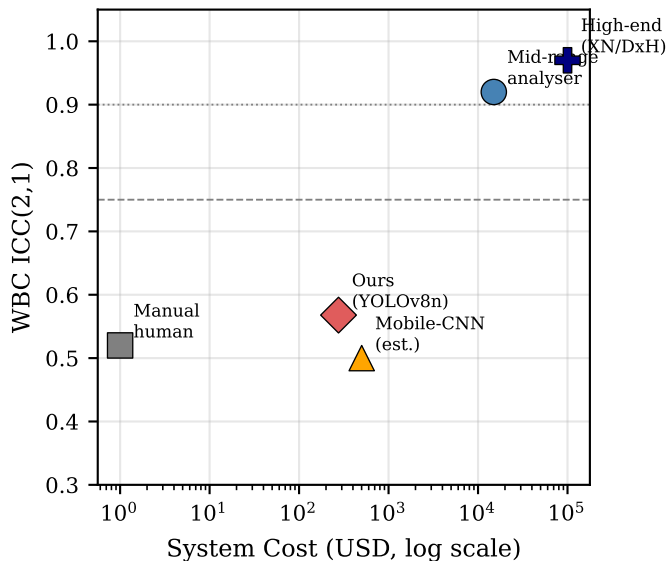
Performance-Cost Frontier: ICC(2,1) vs. System Cost
