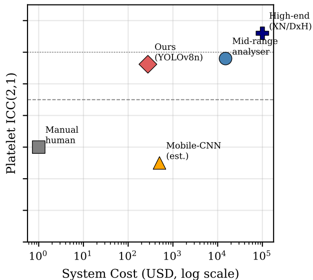
Performance-Cost Frontier: ICC(2,1) vs. System Cost
