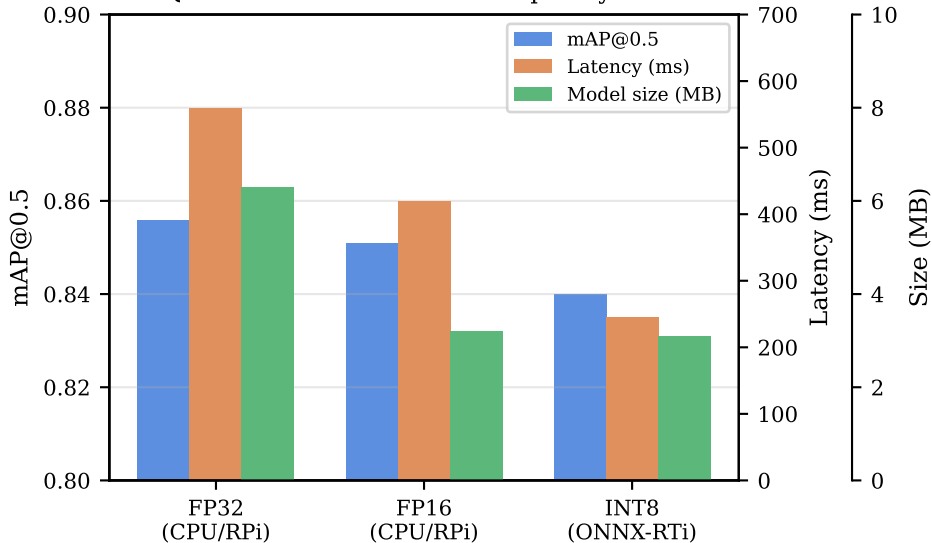
Quantization Trade-off on Raspberry Pi 4B
