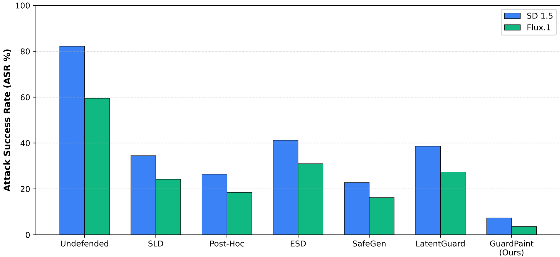
Adversarial Robustness across Defense Baselines
