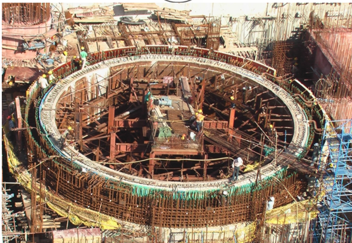
Reactor Vault
