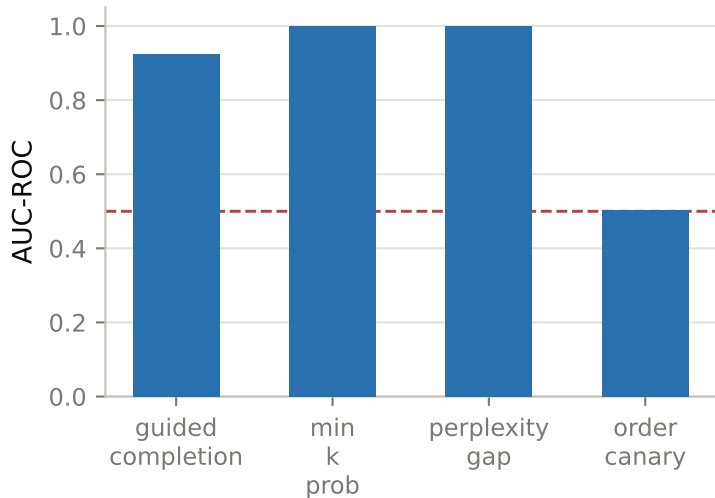
Calibration pilot (n=15, LoRA fine-tune)
