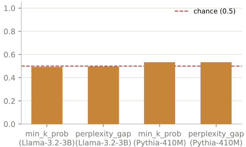
WikiMIA external validation
