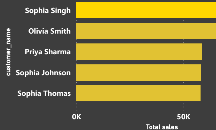
Total sales by customer_name
