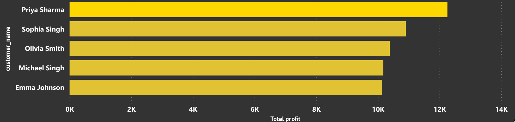
Total profit by customer_name
