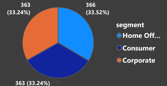
Sales by customer_name by segment
