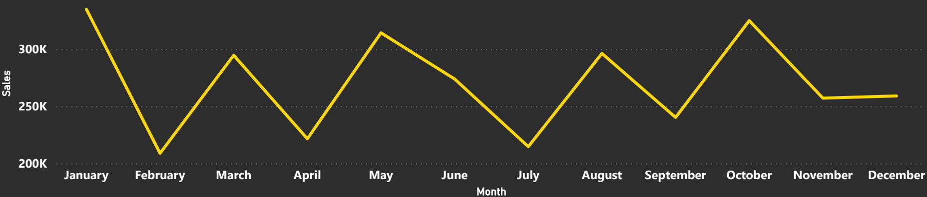
Sales by Month
