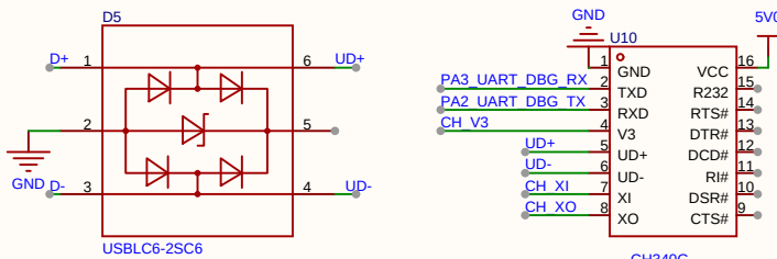
USB转串口CH340G
