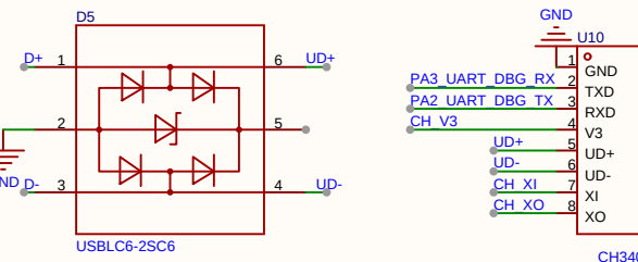
USB转串口CH340G
