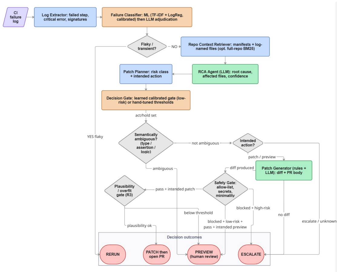
Figure 4.2: The implemented PatchOps pipeline end-to-end. A CI failure log is extracted and classified (TF-IDF + calibrated logistic regression, then LLM adjudication); flaky failures rerun, otherwise the system retrieves repository context, runs root-cause analysis, plans a risk class and intended action, and sets act/hold at the decision gate (learned calibrated gate on the low-risk lane, hand-tuned thresholds elsewhere). A semantic-ambiguity backstop, the safety gate, and the plausibility/overfit gate then route each case into exactly one of four explicit decision outcomes: rerun, patch (open PR), preview (human review), or escalate.
