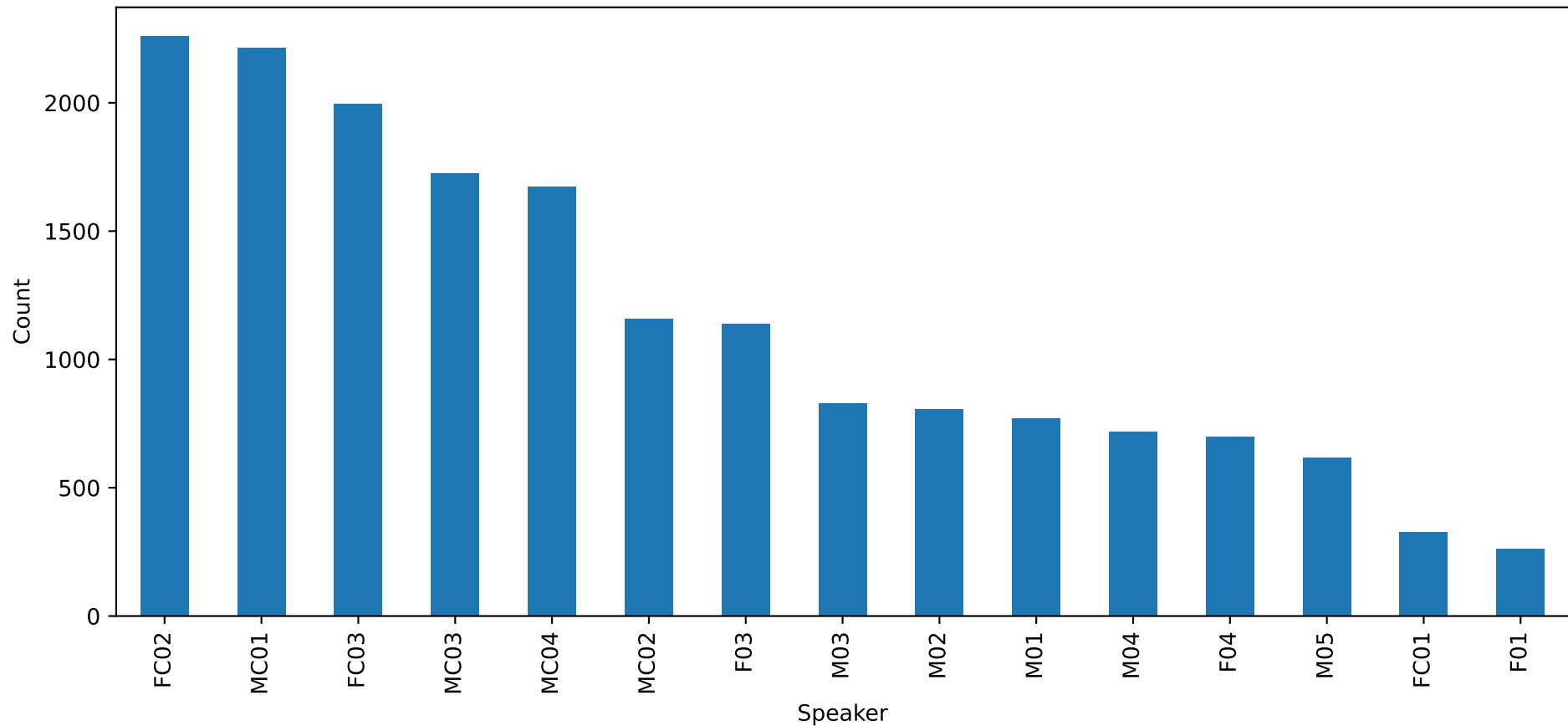
Speaker Distribution
