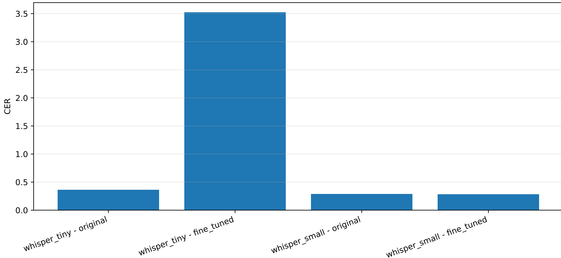
Whisper Tiny vs Small: Original vs Fine-tuned CER
