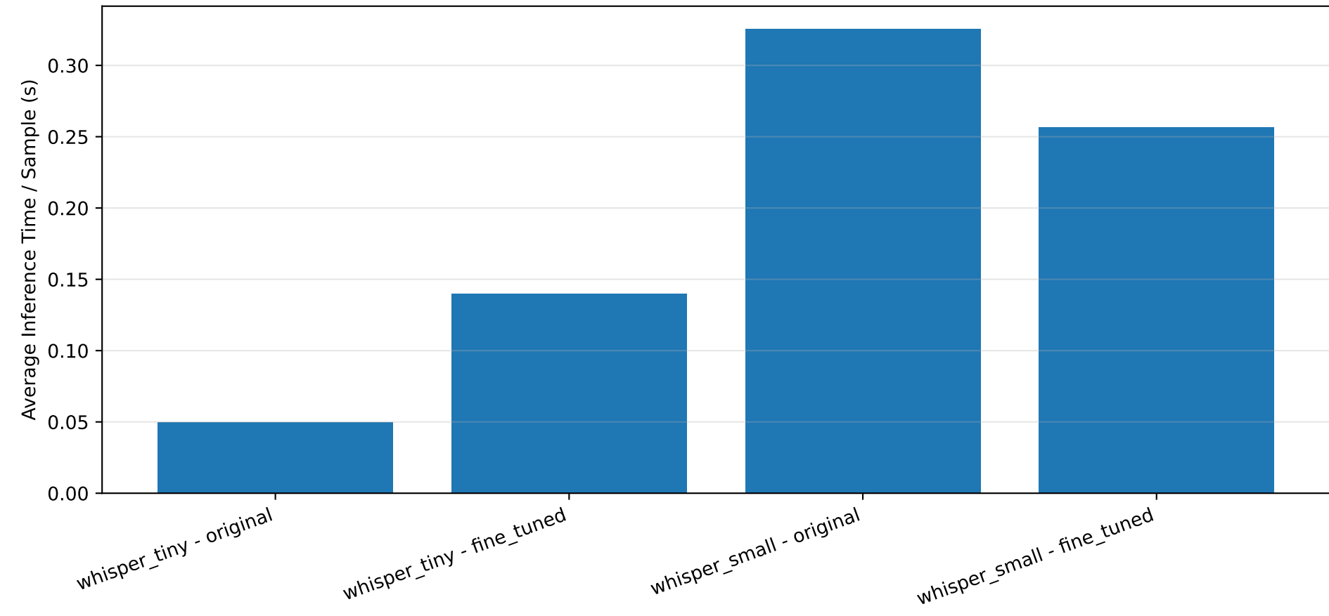
Whisper Runtime Comparison
