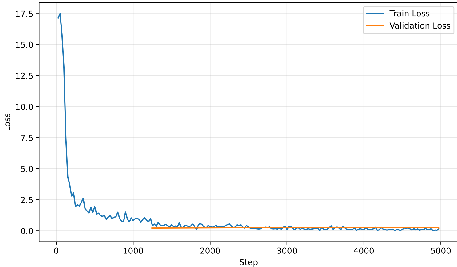
whisper_small Learning Curve
