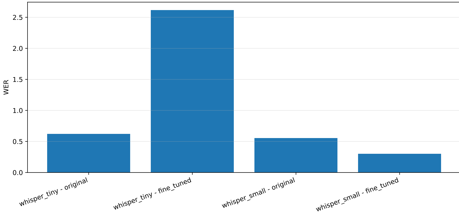
Whisper Tiny vs Small: Original vs Fine-tuned WER
