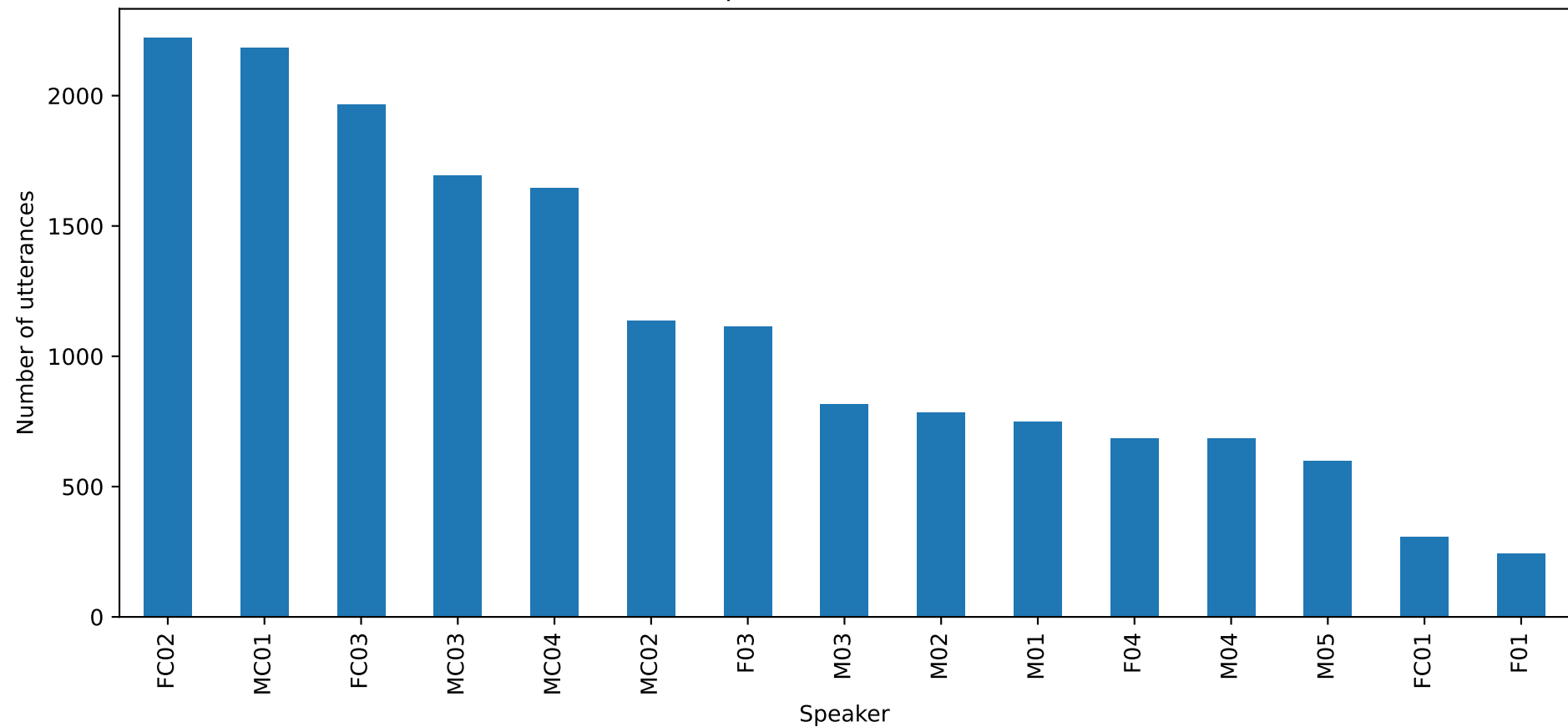
Speaker Distribution
