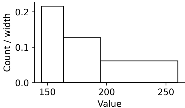
Equal frequency
