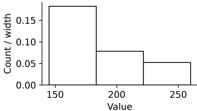
Equal width
