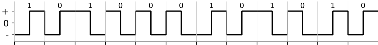
Differential Manchester
