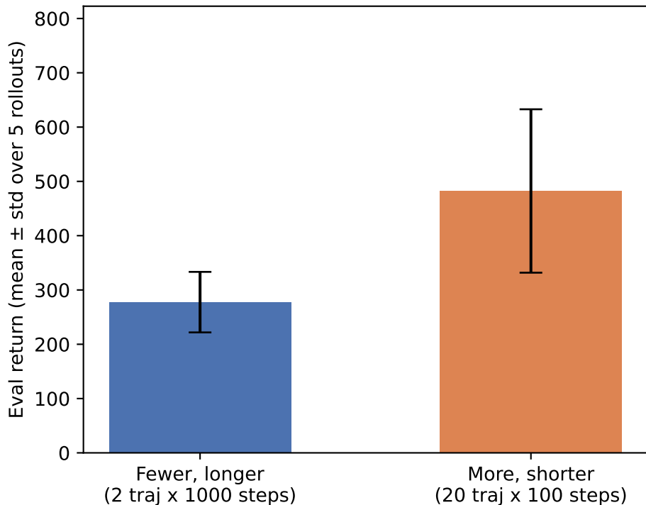
BC on Humanoid-v2: rollout length ablation
