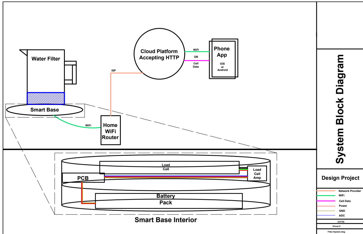
Figure 6: The system block diagram represents the pieces of the device and how they are interconnected.
