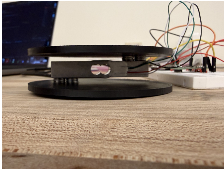
Figure 4: Side view of the assembled prototype showing the two base plates, load cell, and wiring to the microcontroller.
