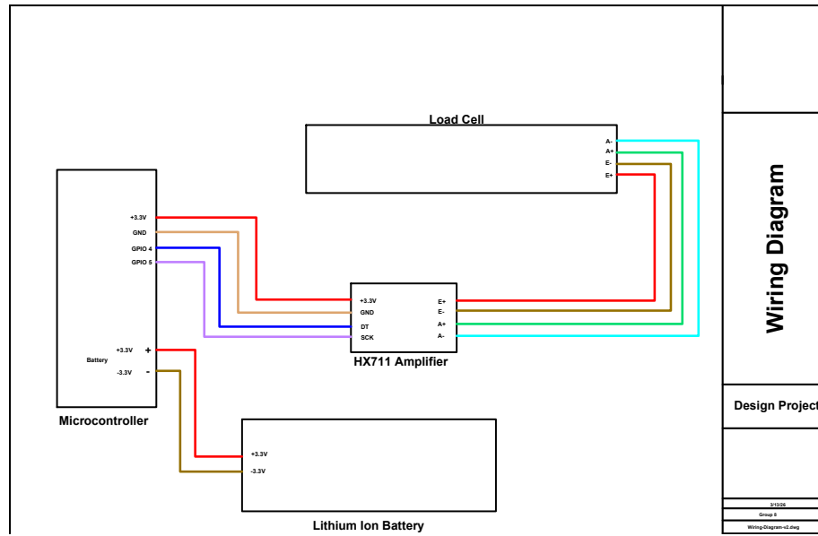
Figure 9: Example Wiring Diagram of Components Included in System Design
