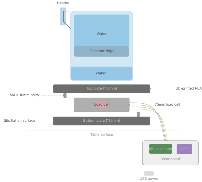
Figure 3: Diagram of the full system assembly showing the water filter pitcher resting on the load cell platform, with wiring to the ESP32 and HX711 on the breadboard.
