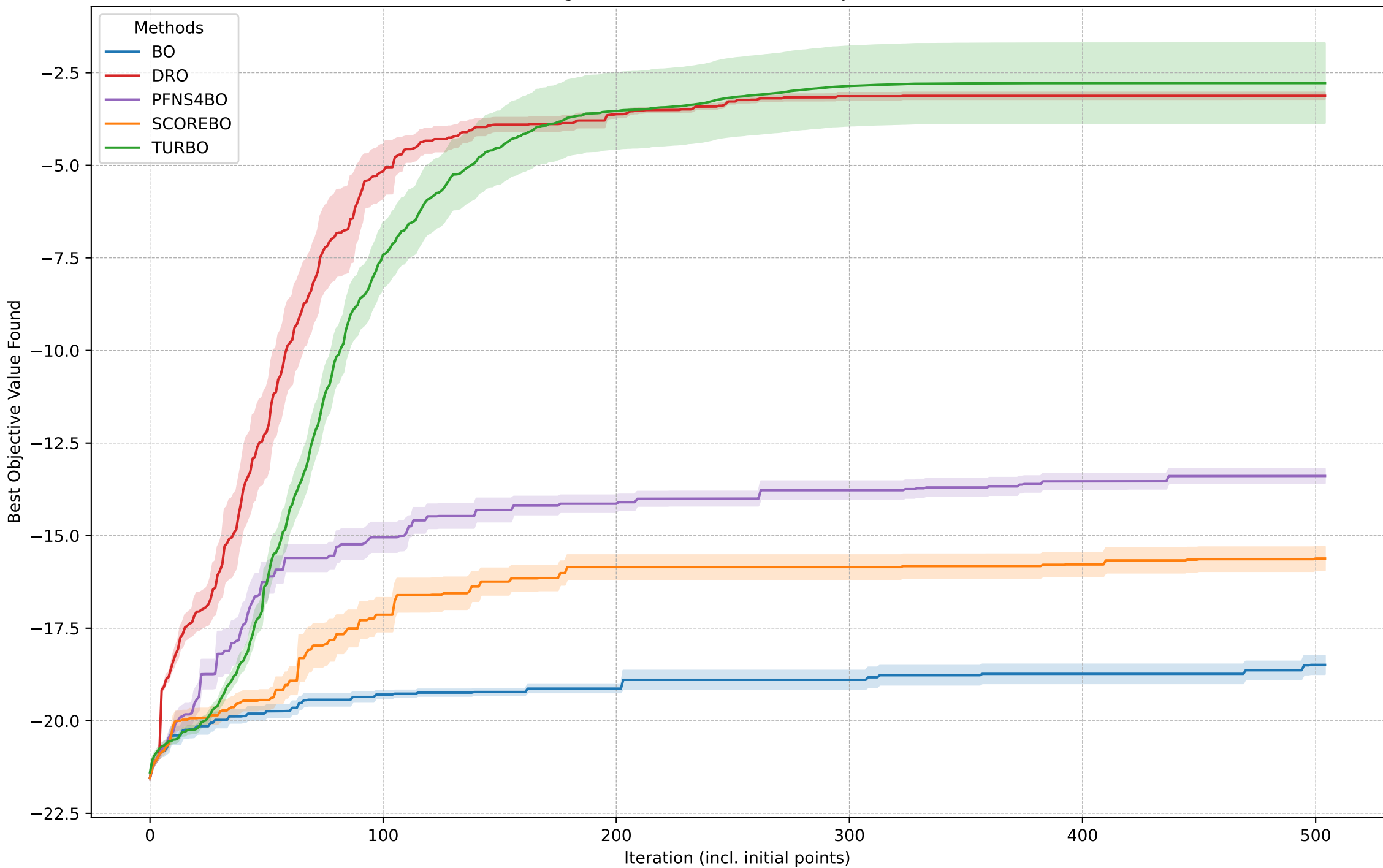
Comparison of Methods on Ackley 10D Average Cumulative Maximum Objective Value
