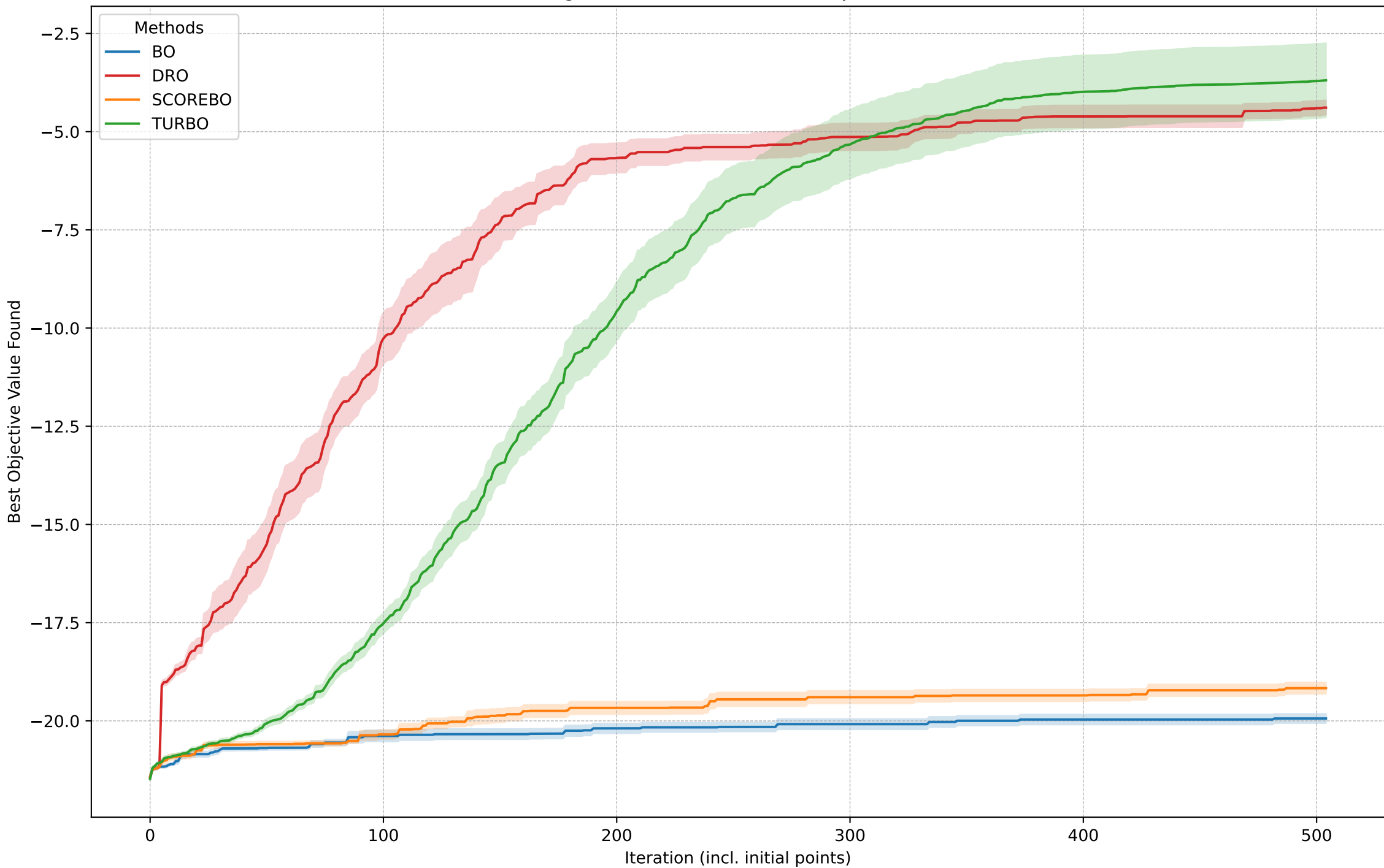
Comparison of Methods on Ackley 20D Average Cumulative Maximum Objective Value
