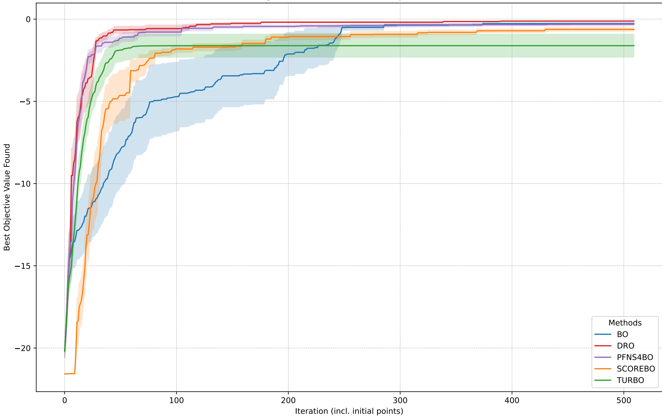
Comparison of Methods on Ackley 2D Average Cumulative Maximum Objective Value
