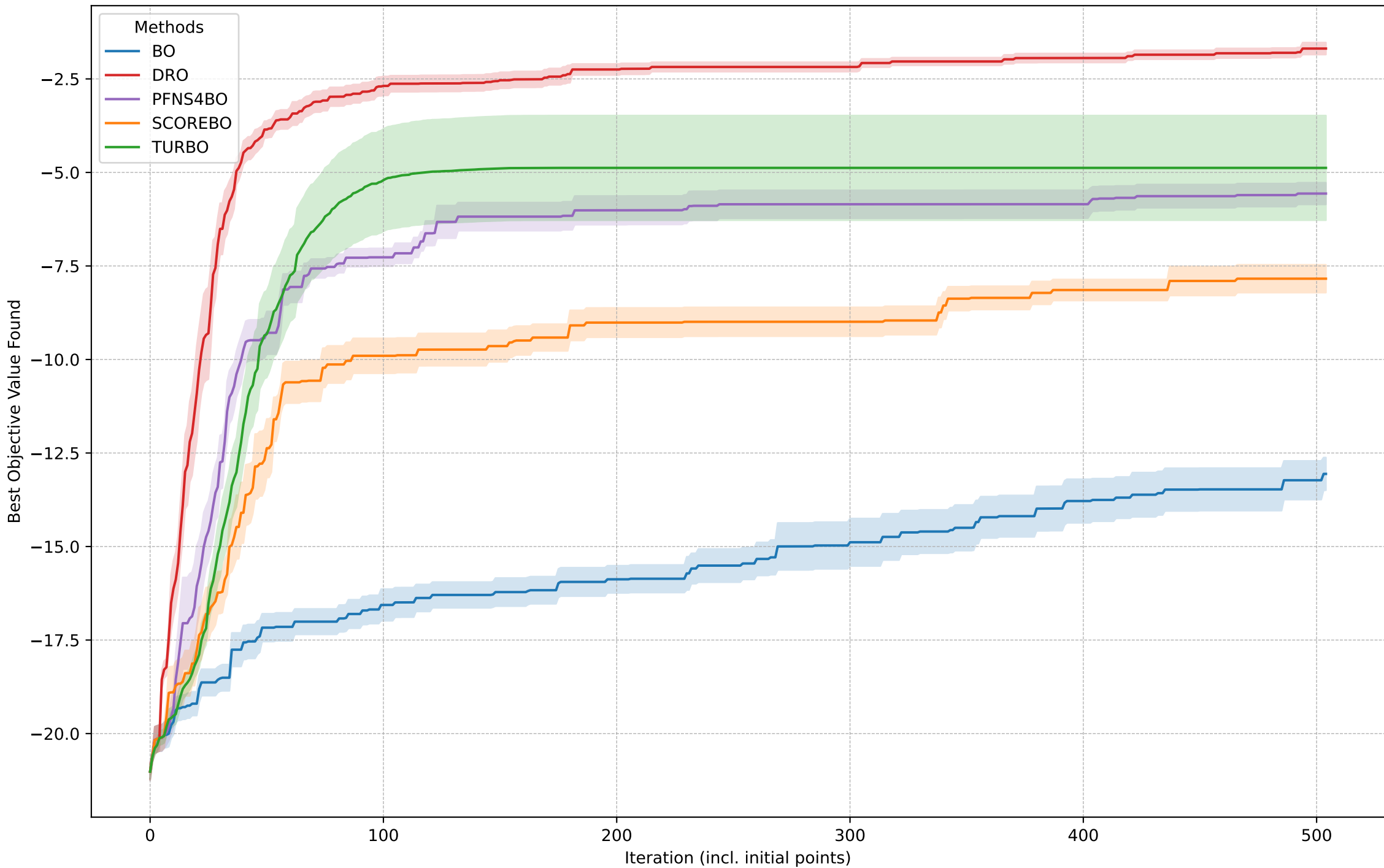
Comparison of Methods on Ackley 5D Average Cumulative Maximum Objective Value
