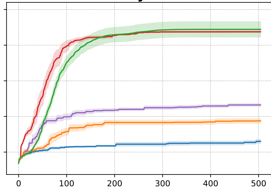
Ackley 10D
