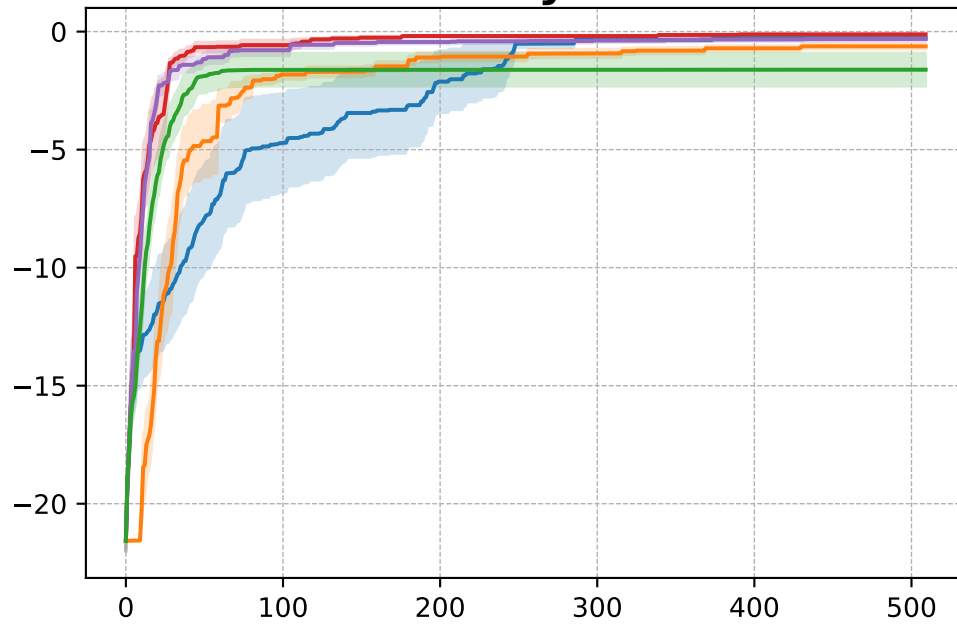
Ackley 2D
