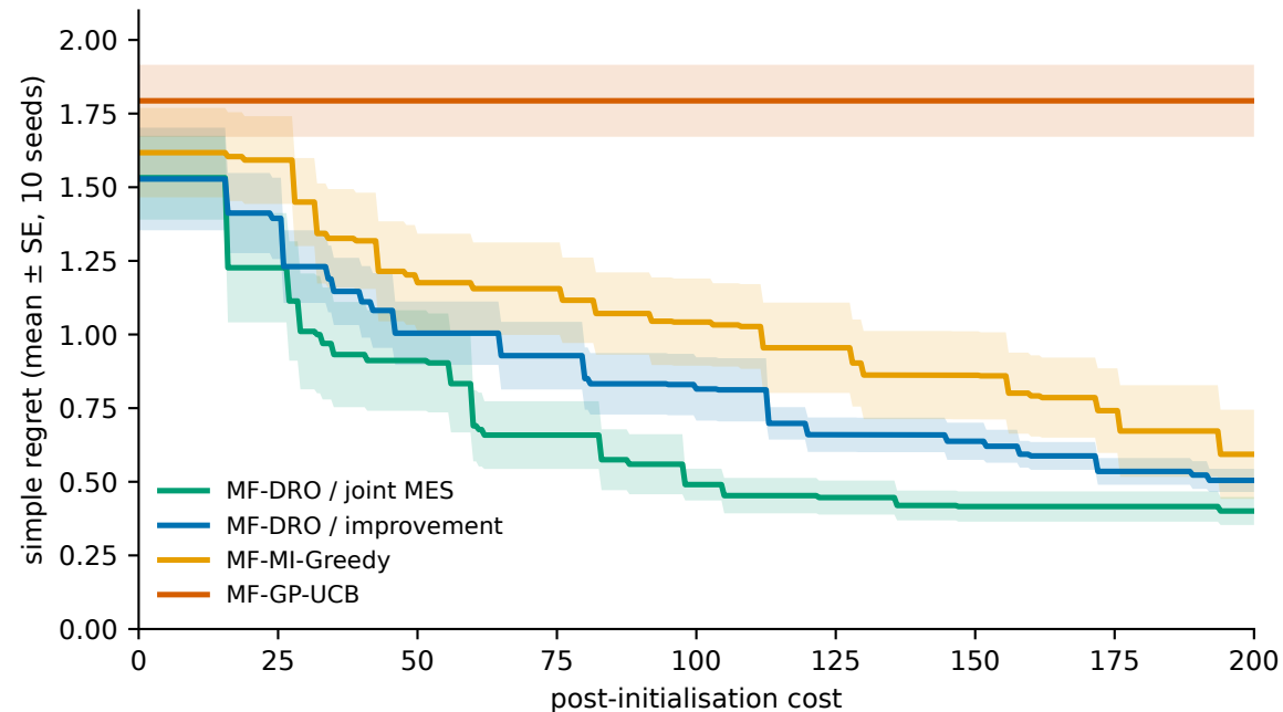
Anytime performance: regret vs cost
