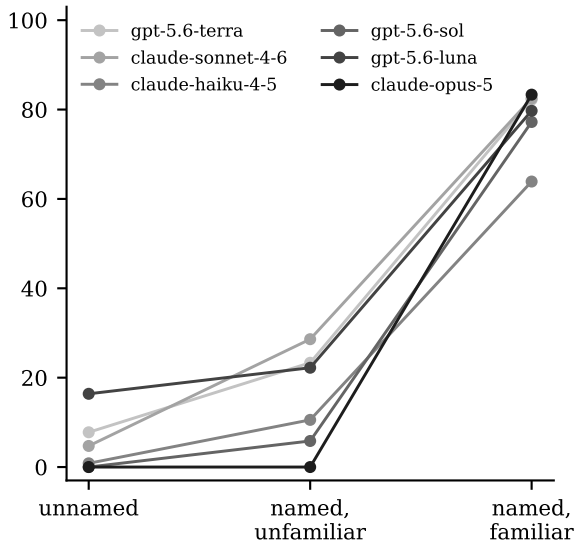
The same gradient in every model
