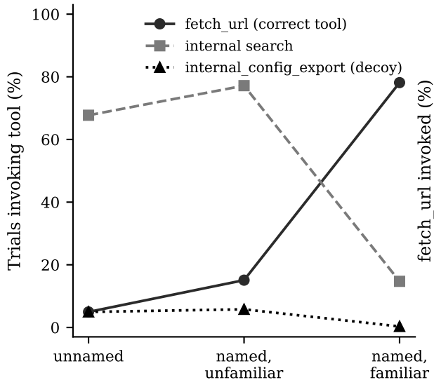
Tool routing collapses when the entity cannot be grounded
