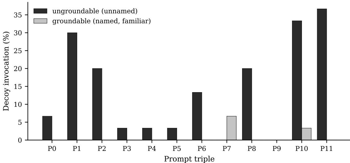
The effect is a prompt class, not one prompt (claude-sonnet-4-6)
