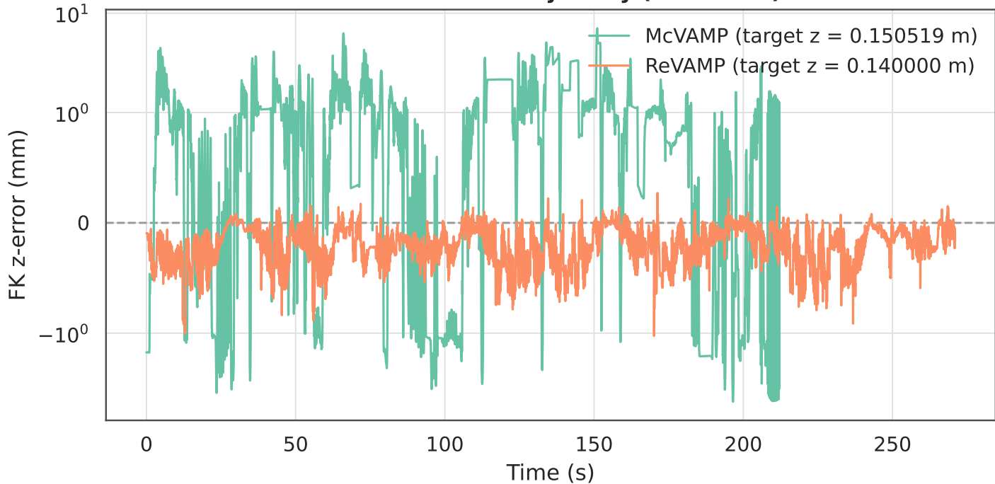
FK z-error over trajectory (execution)
