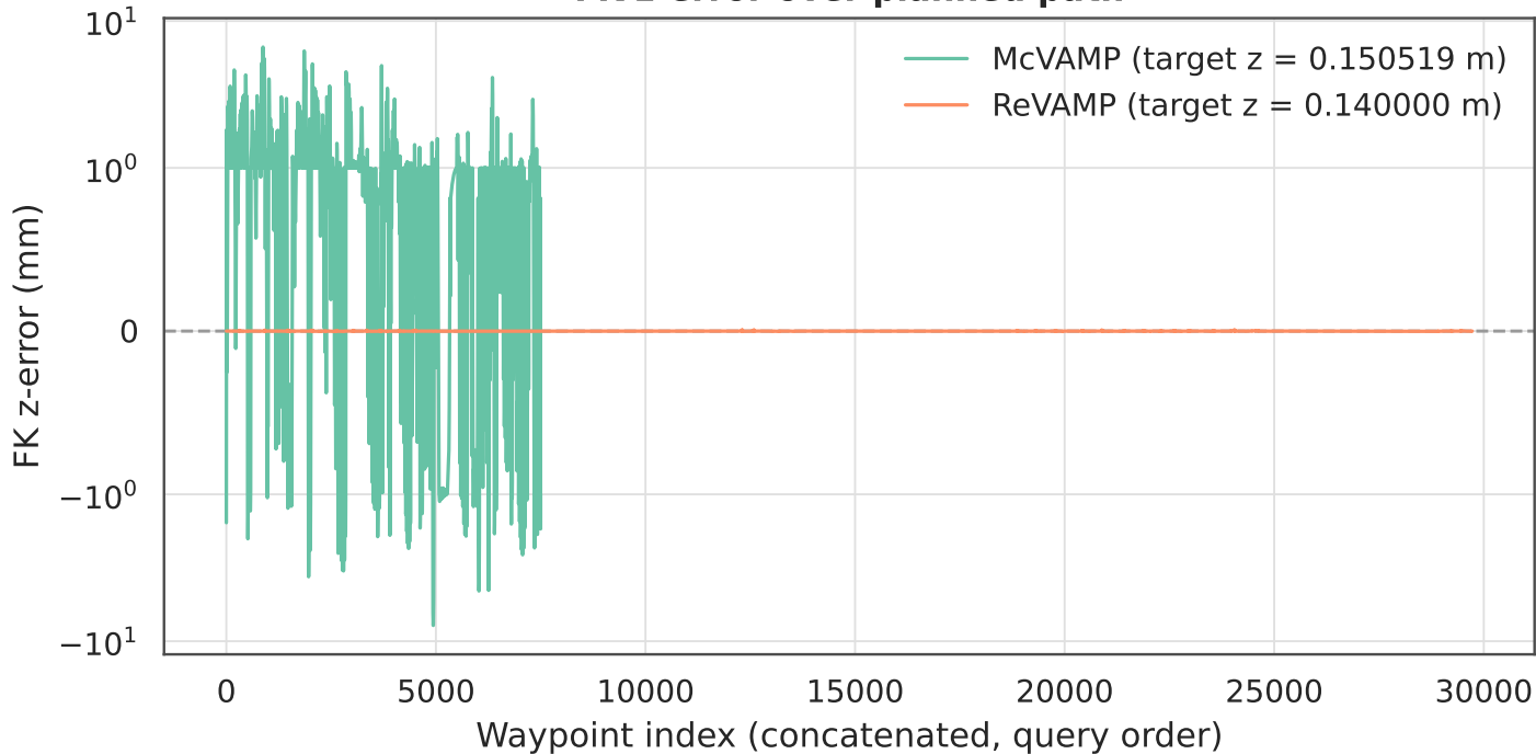
FK z-error over planned path
