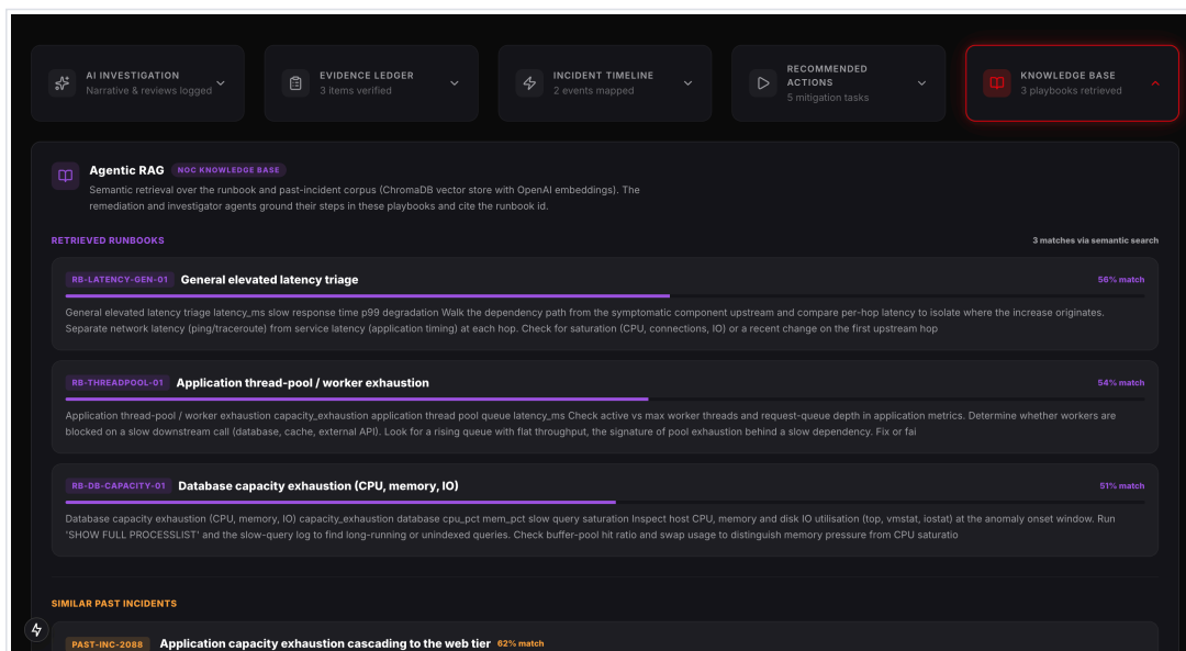
Agentic RAG in the open: runbooks and past incidents retrieved by semantic search over a ChromaDB vector store, each with its similarity score, feeding the agents' grounded and cited output.
