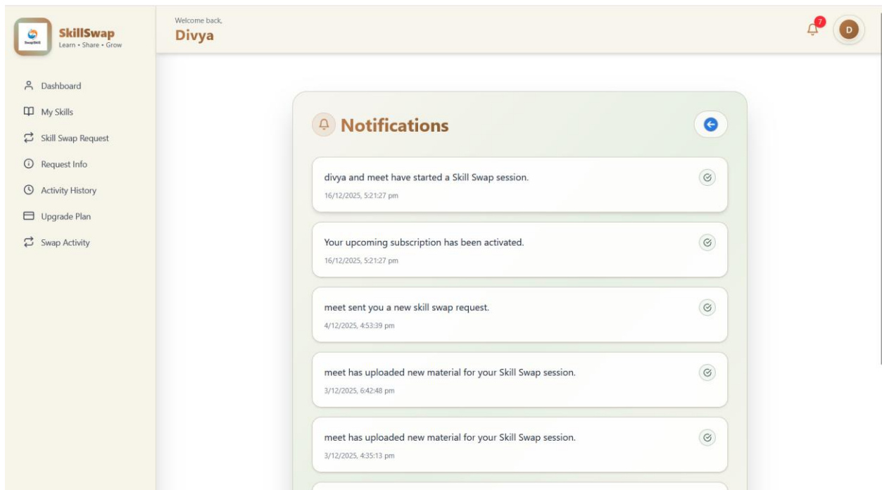
Figure 6.1.19: Notification Page
