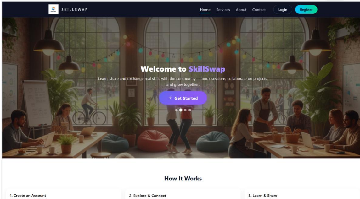
Figure 6.1.1: Home page
