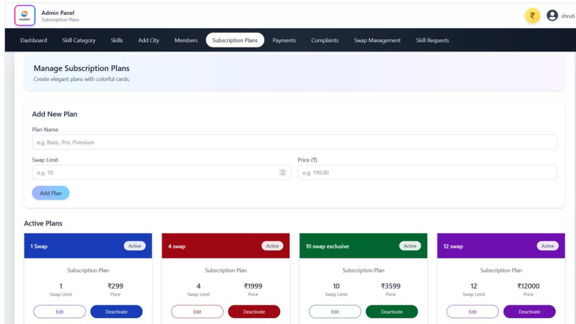
Figure 6.1.9: Subscription page
