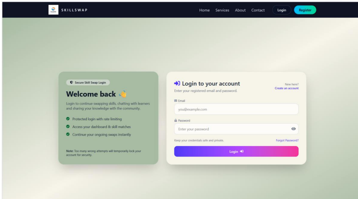
Figure 6.1.3: Login page
