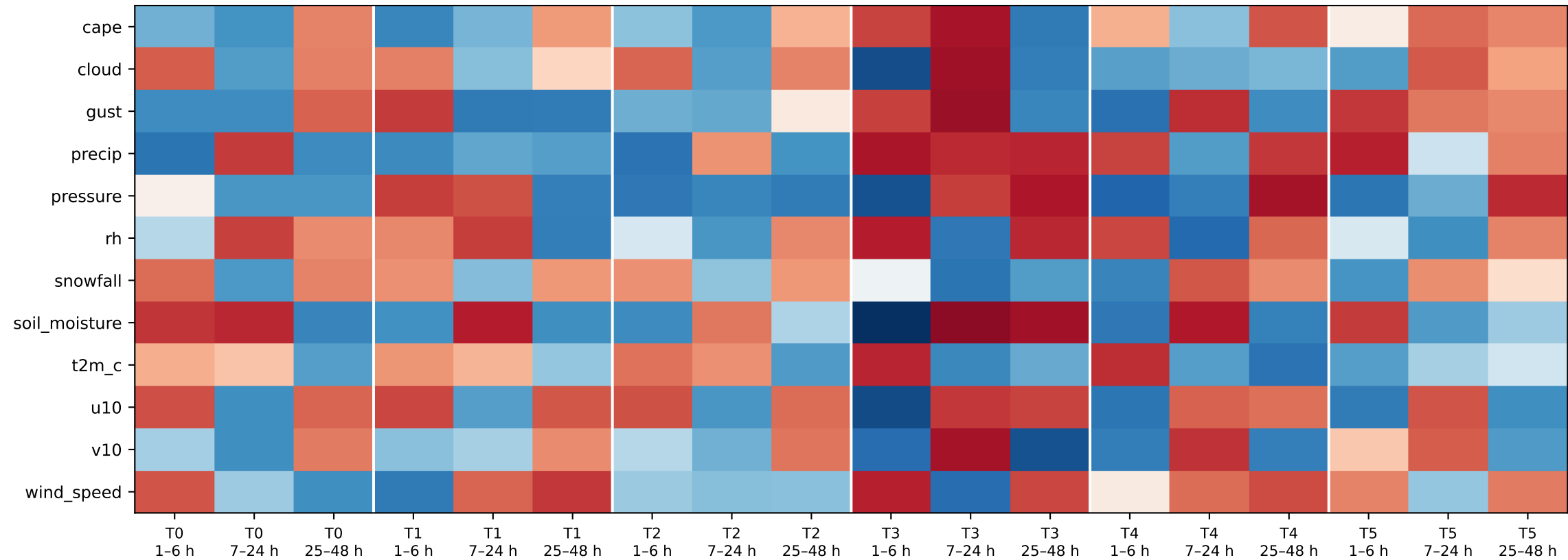
Within approximate joint-history support
