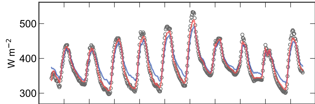
(b) R_{lu}
