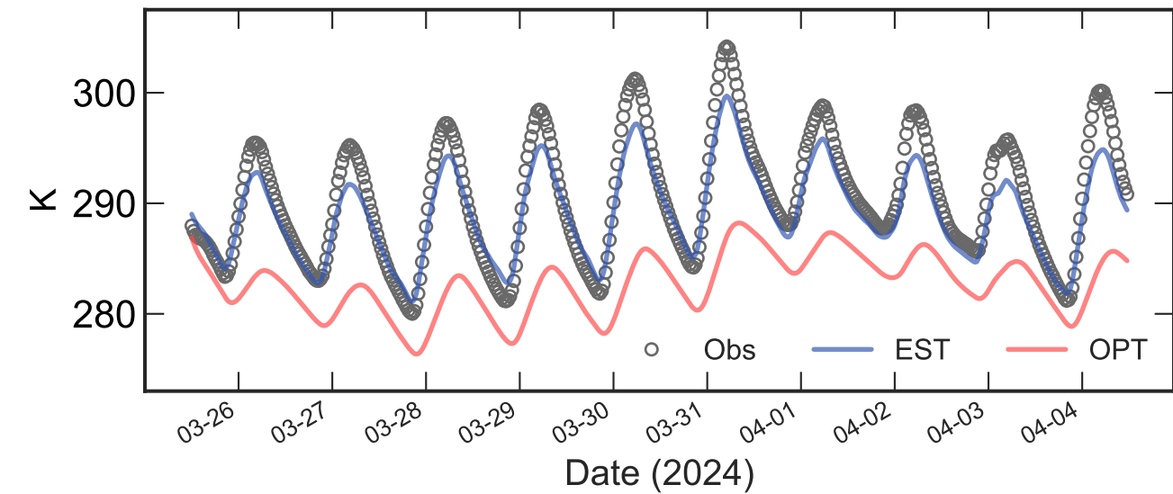
(f) T_{10cm}
