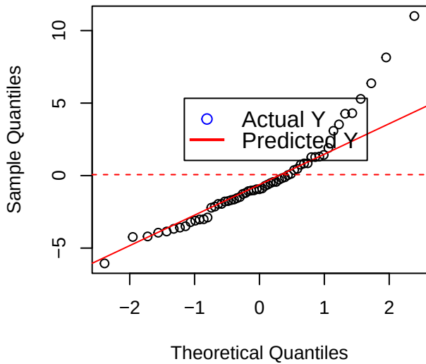
QQ Plot of Deviance Residuals
