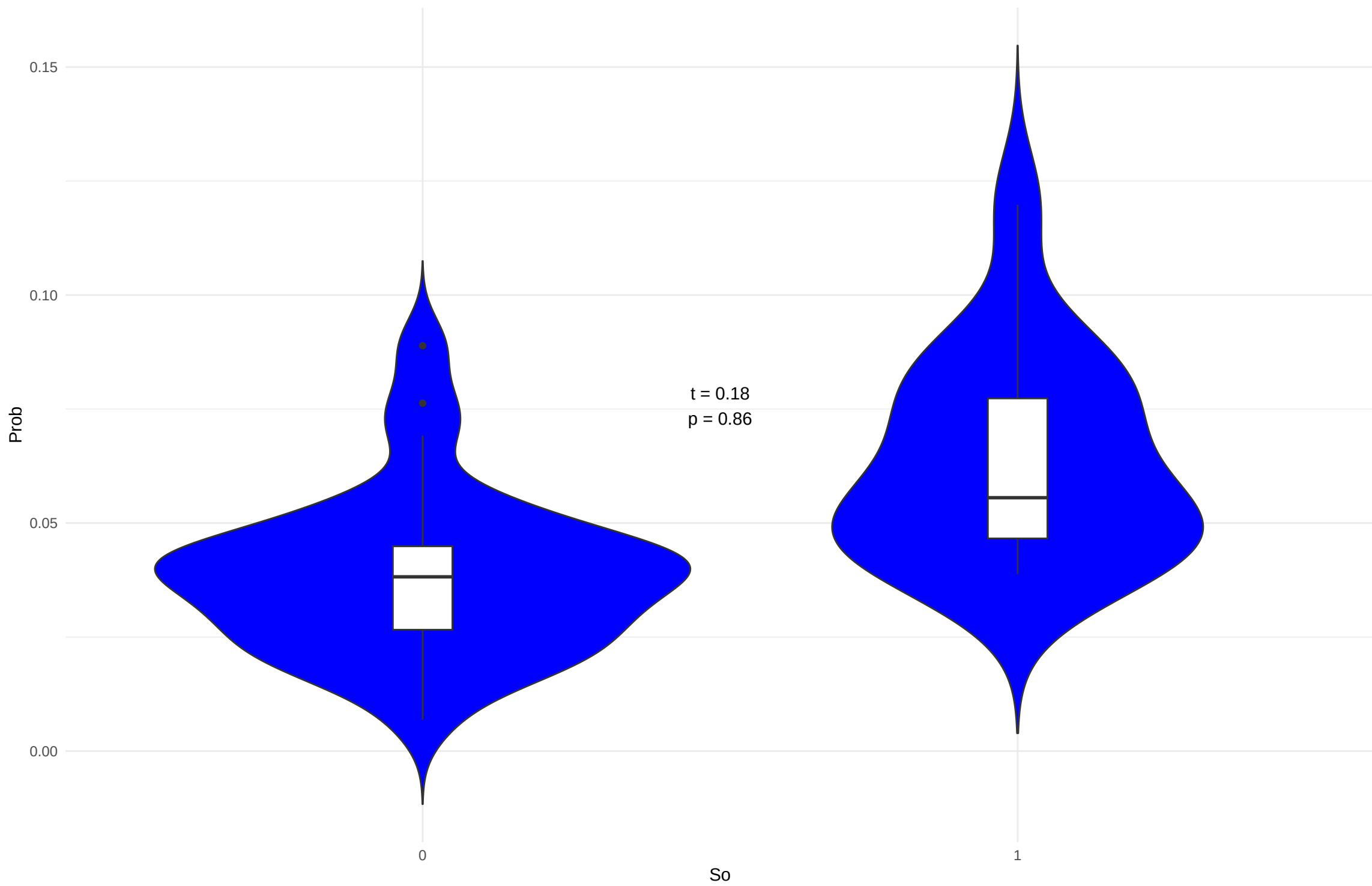
Distribution of Prob by So
