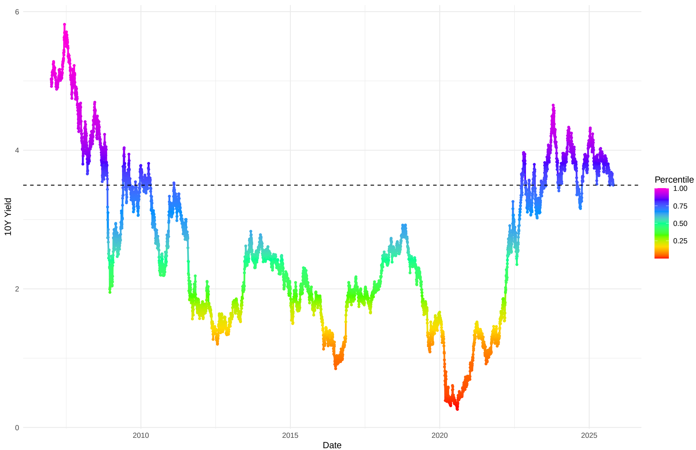
10Y Yield Over Time with Historical Distribution
