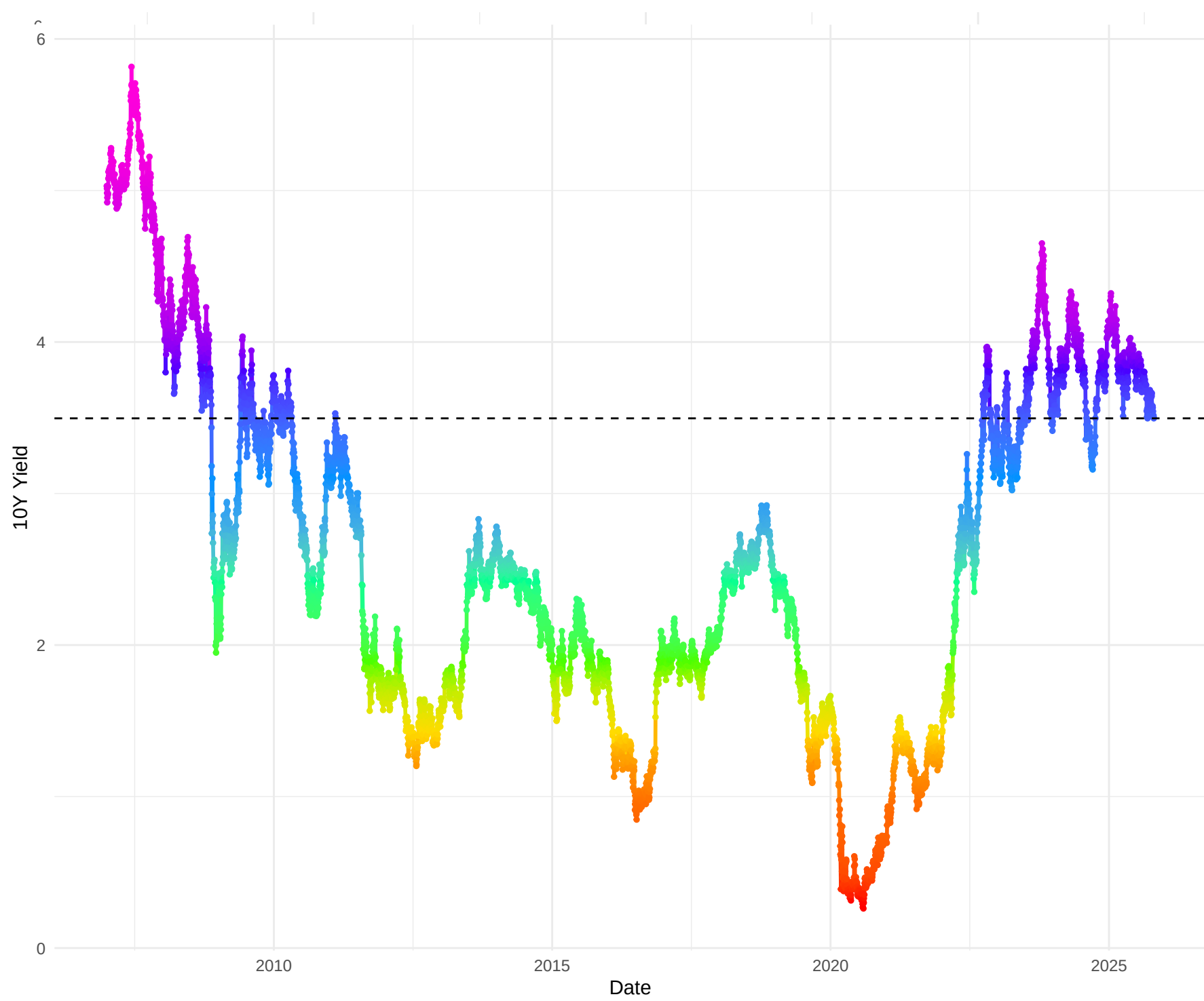
10Y Yield Over Time with Historical Distribution
