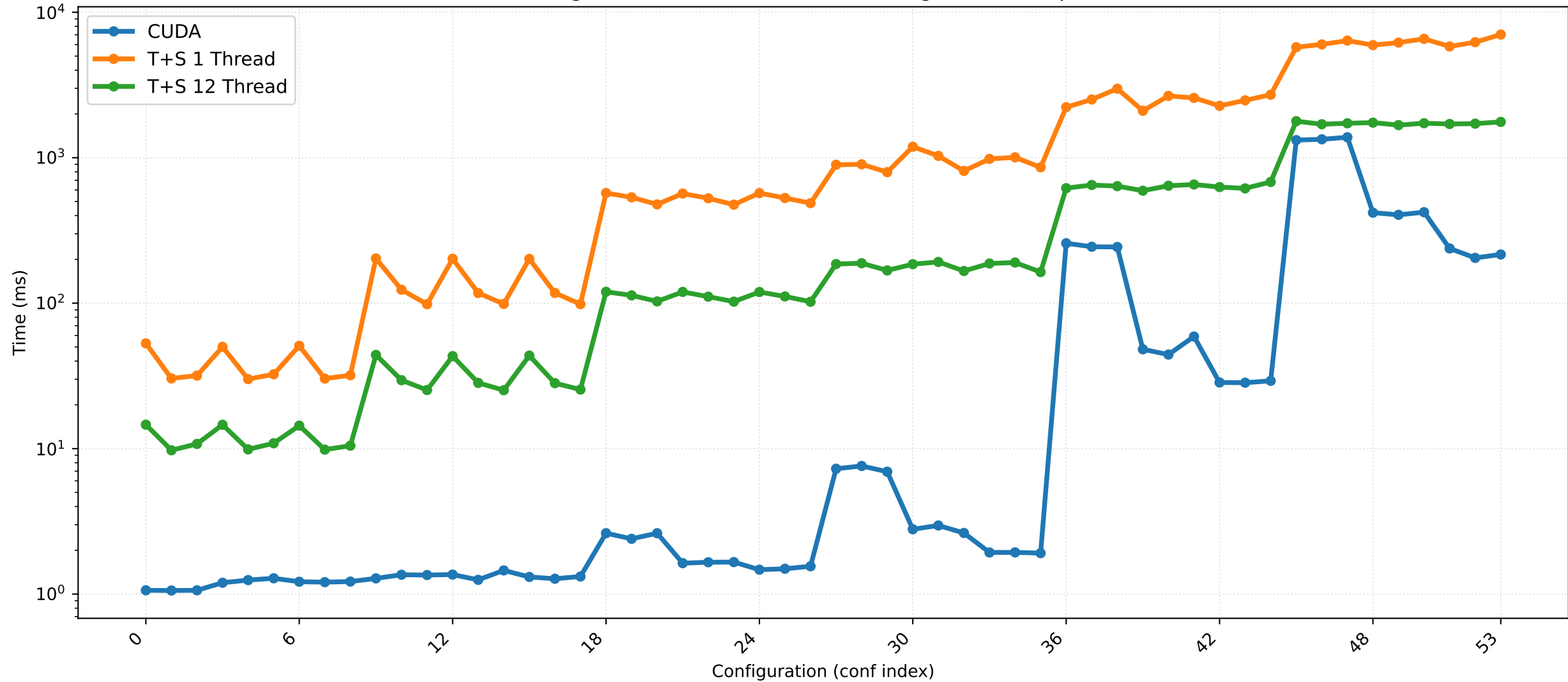
Average Reconstruction (ms) - Per-Configuration Comparison
