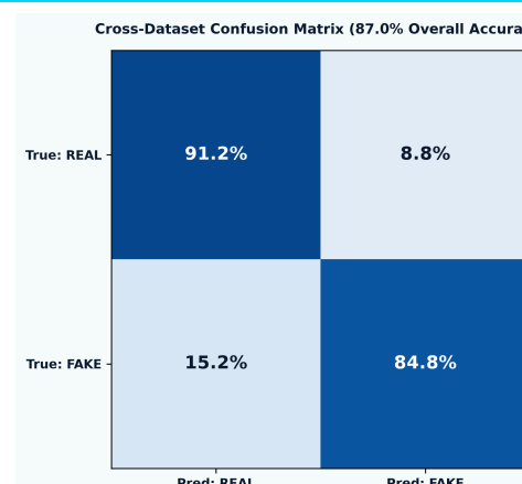
Figure 3: Cross-Dataset Confusion Matrix (True Real: 91.2%, True Fake: 84.8%).
