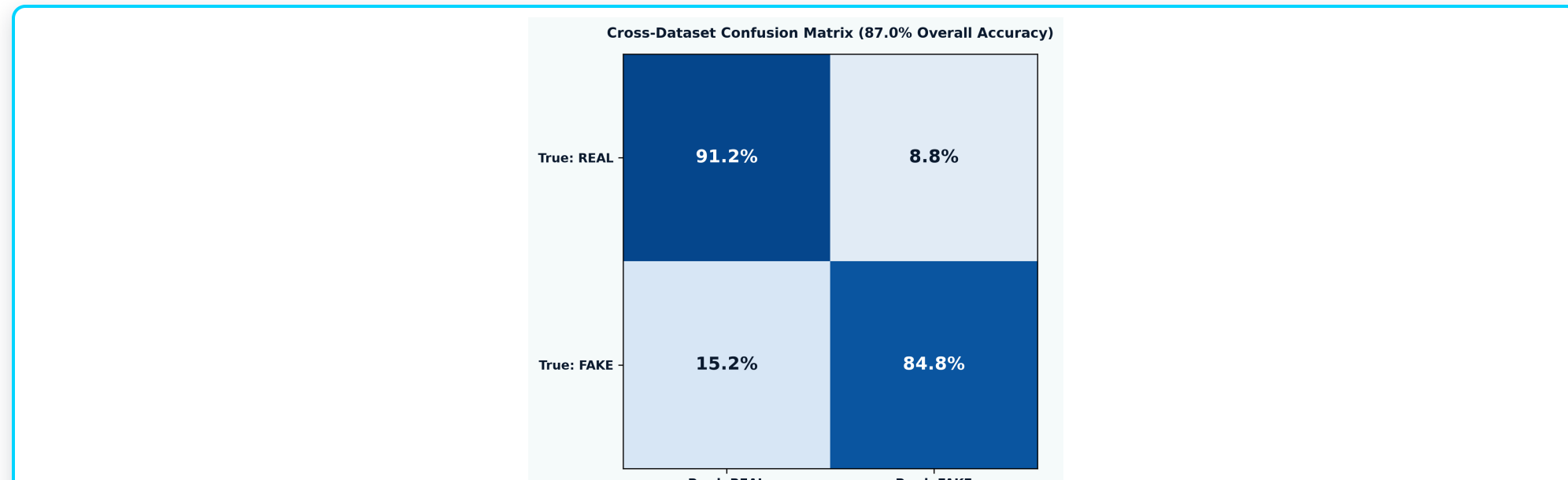
Figure 3: Cross-Dataset Confusion Matrix (True Real: 91.2%, True Fake: 84.8%).
