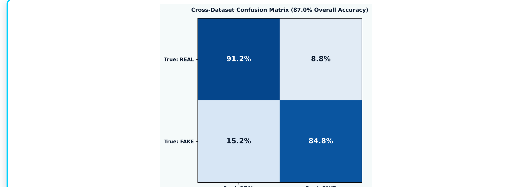
Figure 3: Cross-Dataset Confusion Matrix (True Real: 91.2%, True Fake: 84.8%).
