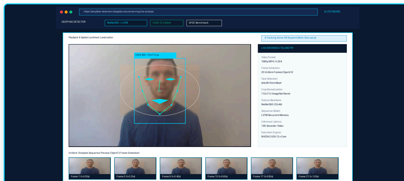
Figure 2 (UI Snapshot 1): Real-Time Web Video Screening & 68-Keypoint Facial Tracking. Browser-based face-api.js mesh tracks inter-frame spatial boundaries before ResNeXt50+LSTM temporal inference.
