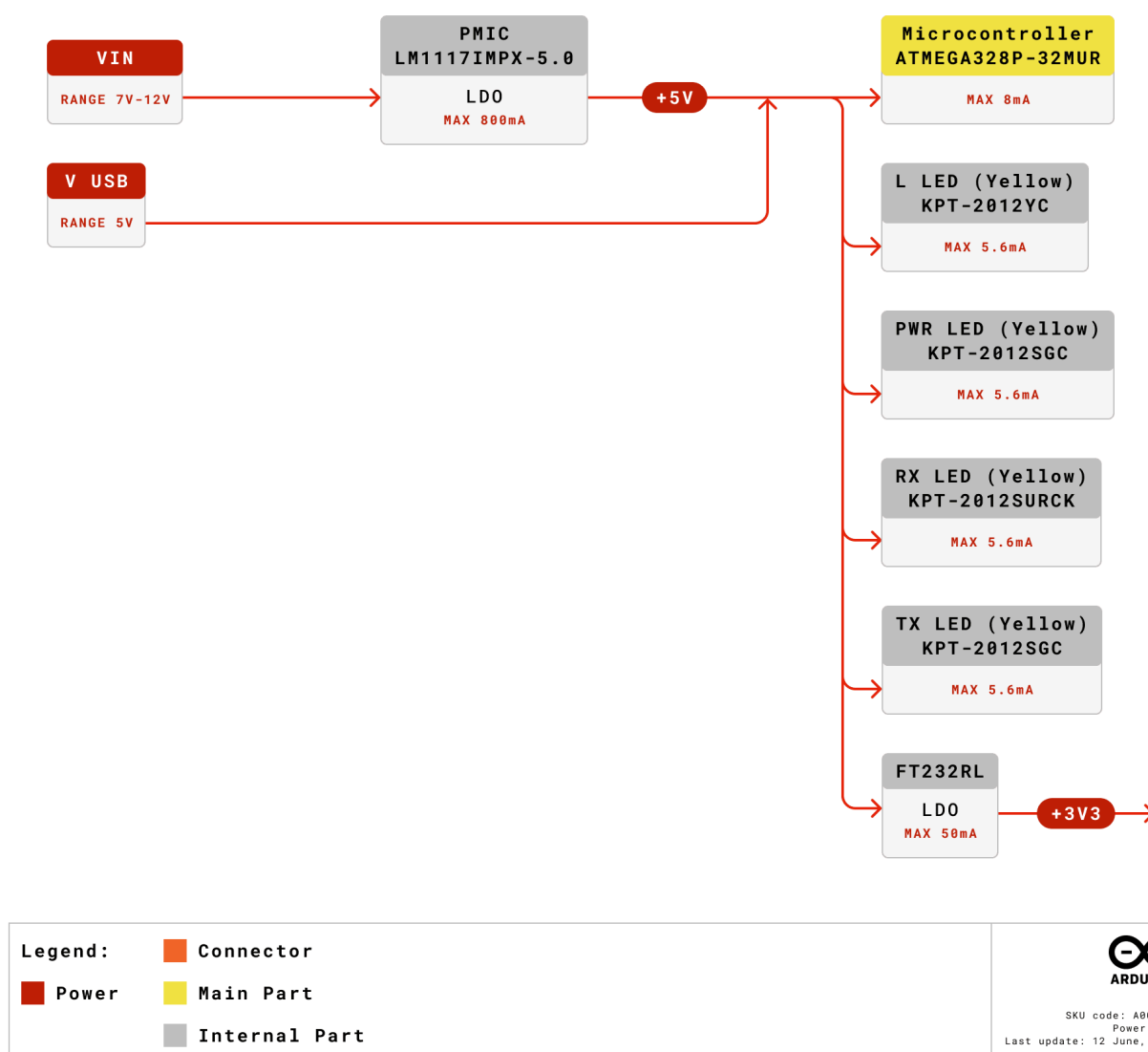
Power Tree of Arduino Nano
