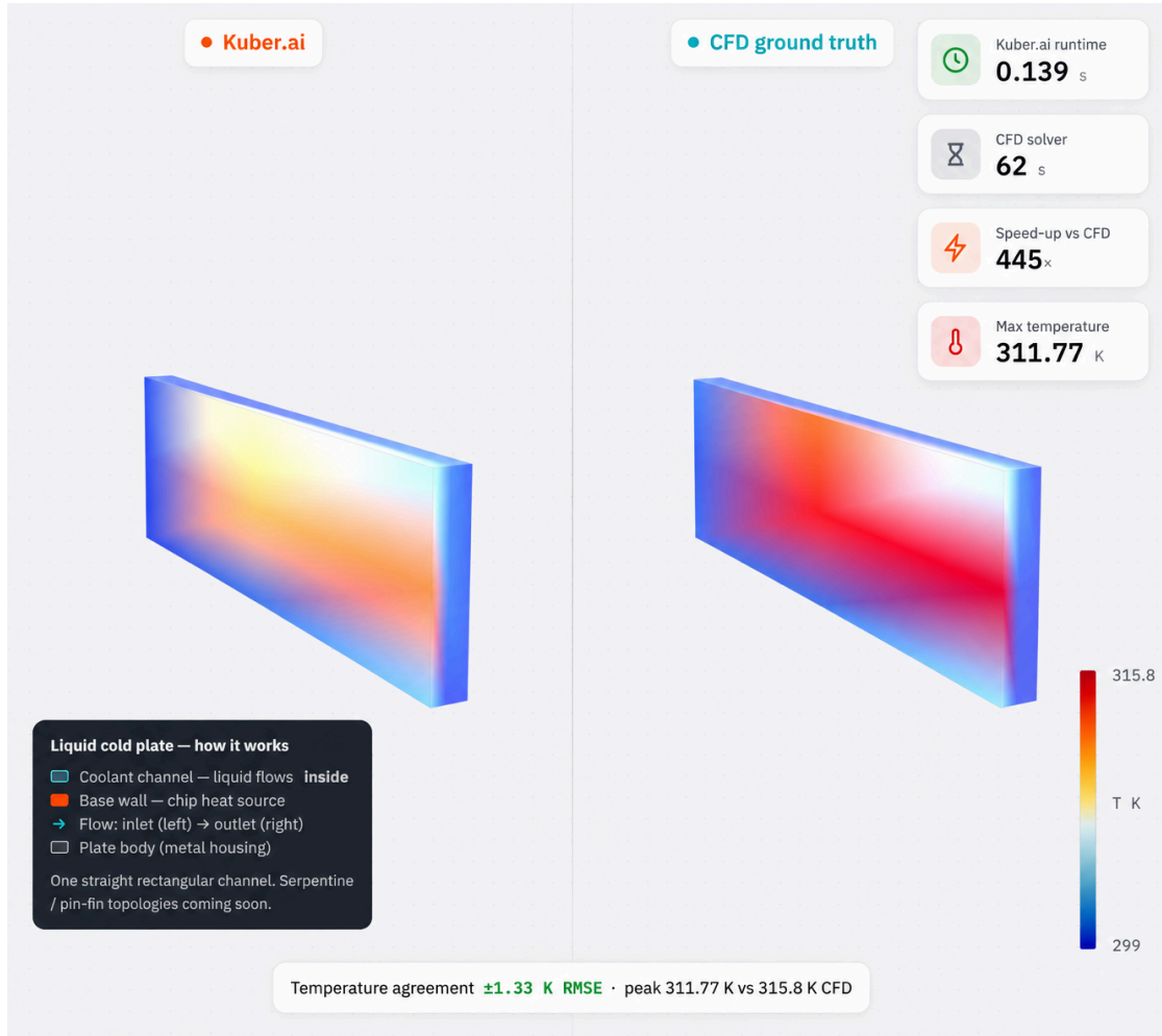
Fig. 3. Kuber prediction vs. CFD ground truth for a liquid cold plate: surface temperature field, \pm 1.33 K RMSE agreement (peak 311.77 vs. 315.8 K CFD), computed 445 \times faster than the CFD solver.
