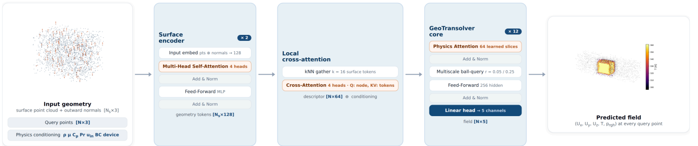
Fig. 2. KuberNet. Three inputs — the boundary surface point cloud with normals, the query points, and the physics conditioning — feed a neural spine (surface encoder \rightarrow local anisotropic boundary-layer (ABL) cross-attention \rightarrow concatenated per-node embedding \rightarrow GeoTransolver physics-attention core) that predicts the five-channel field at every query node.
