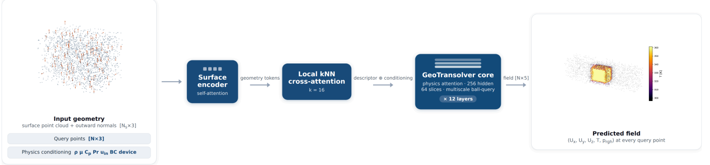
Fig. 2. SurfaceGeoTransolver. Three inputs — the boundary surface point cloud with normals, the query points, and the physics conditioning — feed a neural spine (surface encoder → local kNN cross-attention → concatenated per-node embedding → GeoTransolver physics-attention core) that predicts the five-channel field at every query node.
