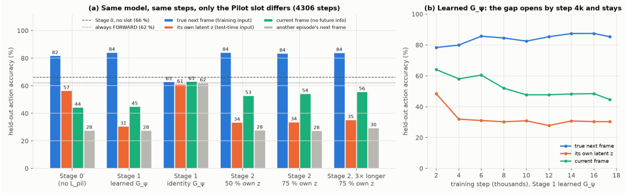
Figure 5: The Pilot-slot shortcut, measured. (a) Held-out action accuracy of each checkpoint with only the slot content changed. (b) The learned Stage 1 model over training: own-latent accuracy collapses by step 4k and stays low while next-frame accuracy stays high.
